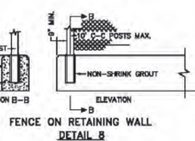
FENCE ON RETAINING WALL DETAIL 8
