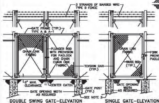
SWINGING GATES DETAIL 4
