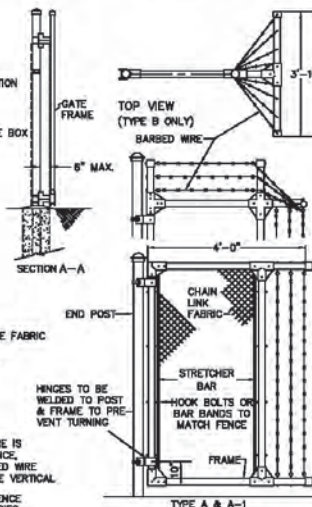
FAN GUARD - TYPE A, A-1 & B FENCE DETAIL 6
